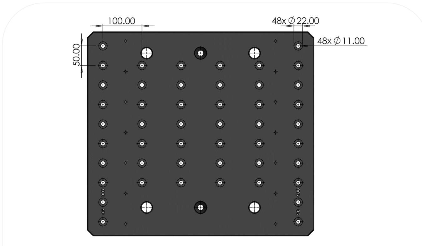
Figure 7: Mounting interfaces of the 8U and 16U TestPod
