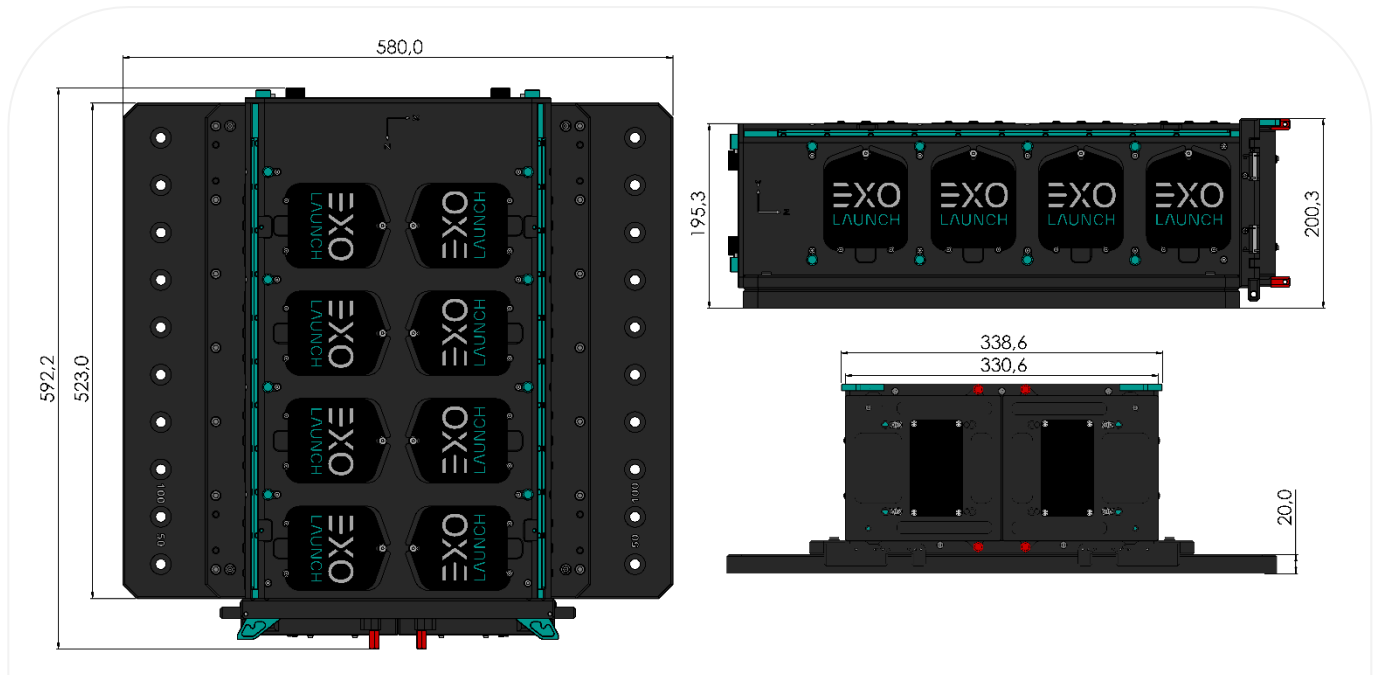
Figure 4: Outer envelope of the 8U TestPod
